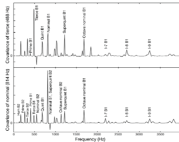
Figure 2. Two rows of the covariance matrix.
